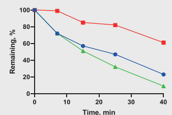
Figure 1. Stability data for benzocaine and analogs in human liver microsomes. “No cofactor” control data indicates some instability of the compound in the test system without cofactors
