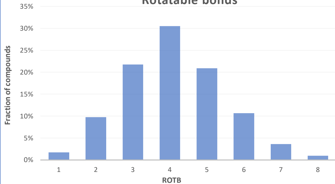
Rotatable bonds
