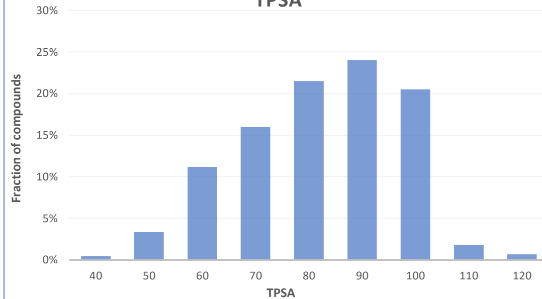
TPSA
