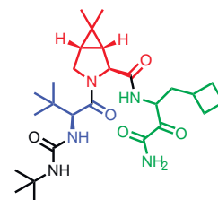
Boceprevir antiviral drug
